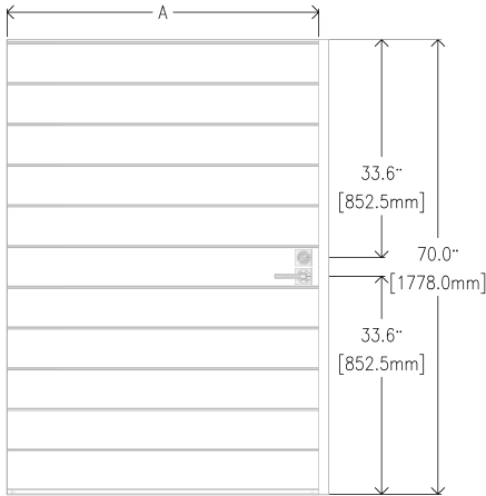
ELEVATION — FRONT
