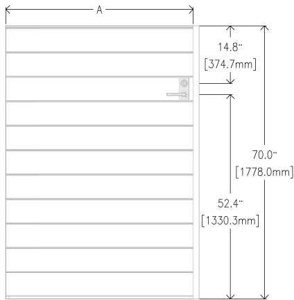
ELEVATION — FRONT
